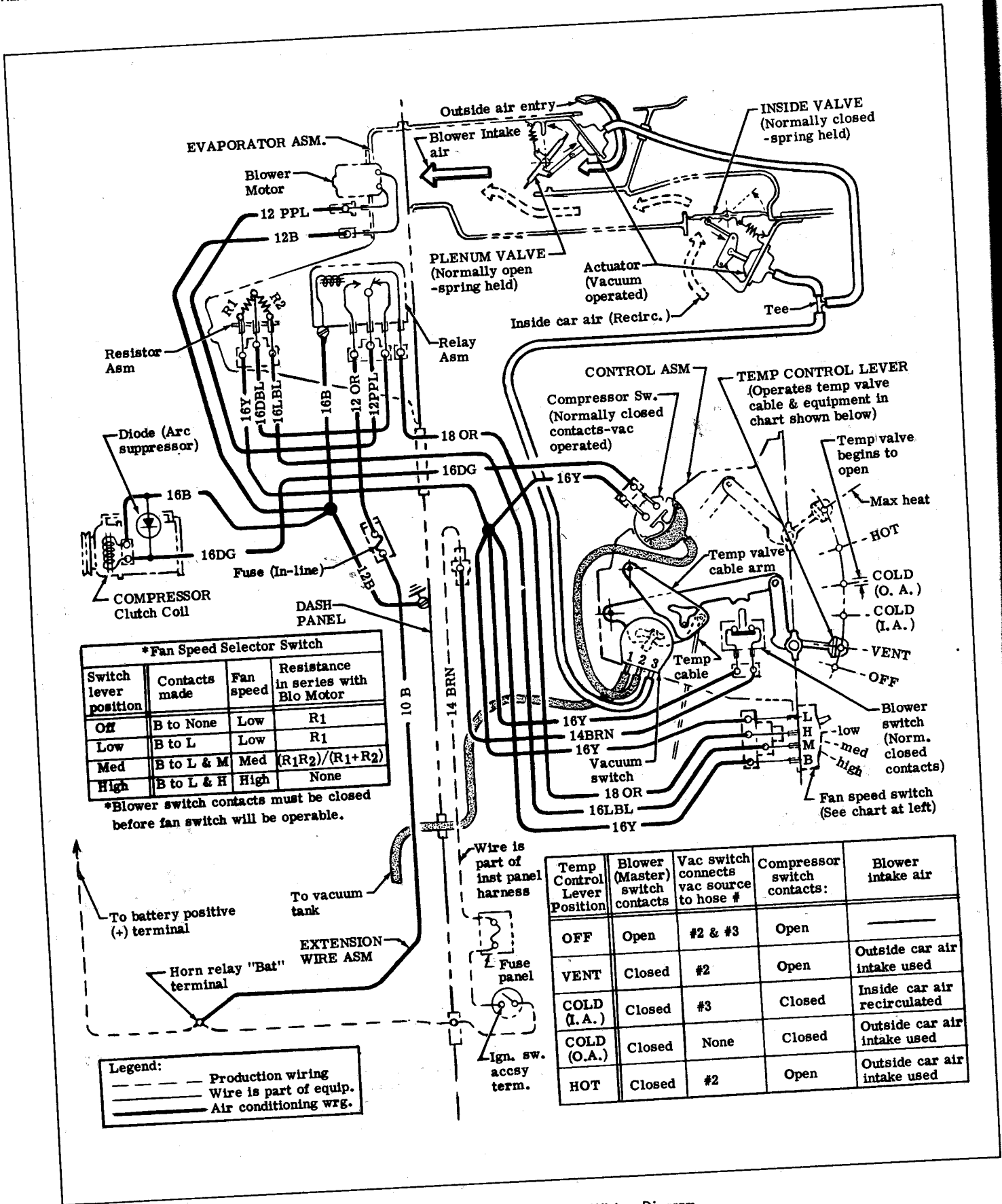
Fig. 116—Camaro—Four-Season Wiring Diagram
