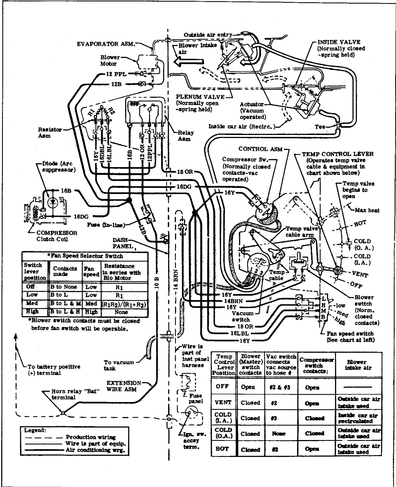
Camaro—Four-Season Wiring Diagram
